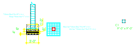
column cross section
