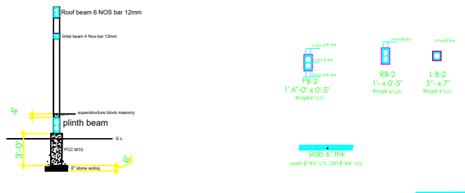
wall cross section
